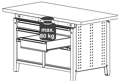
Drawers with single extension E 80 80% extension, 80 kg loading capacity
