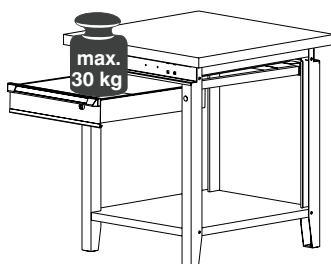
Middle drawers 80% extension, 30 kg loading capacity
